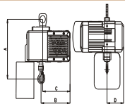
Hoist - 500 with Fixed Suspension
