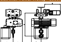
Hoist with Power Trolley - 1600Kg
