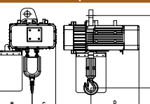
Hoist with Fixed Suspension - 3200Kg
