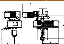
Hoist with Power Trolley - 3200Kg
